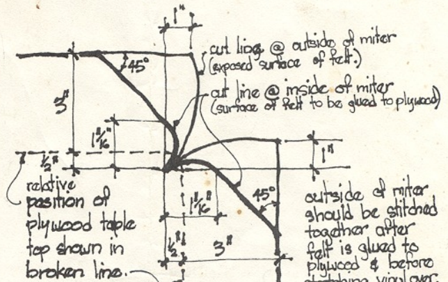
TYPICAL PLAN DETAIL OF CORNER SHOWING FELT MITER CUT.
